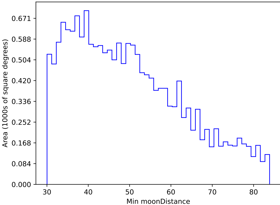
ddf_loaded_fl8_v3.4_10yrs WFD u band: Min moonDistance
