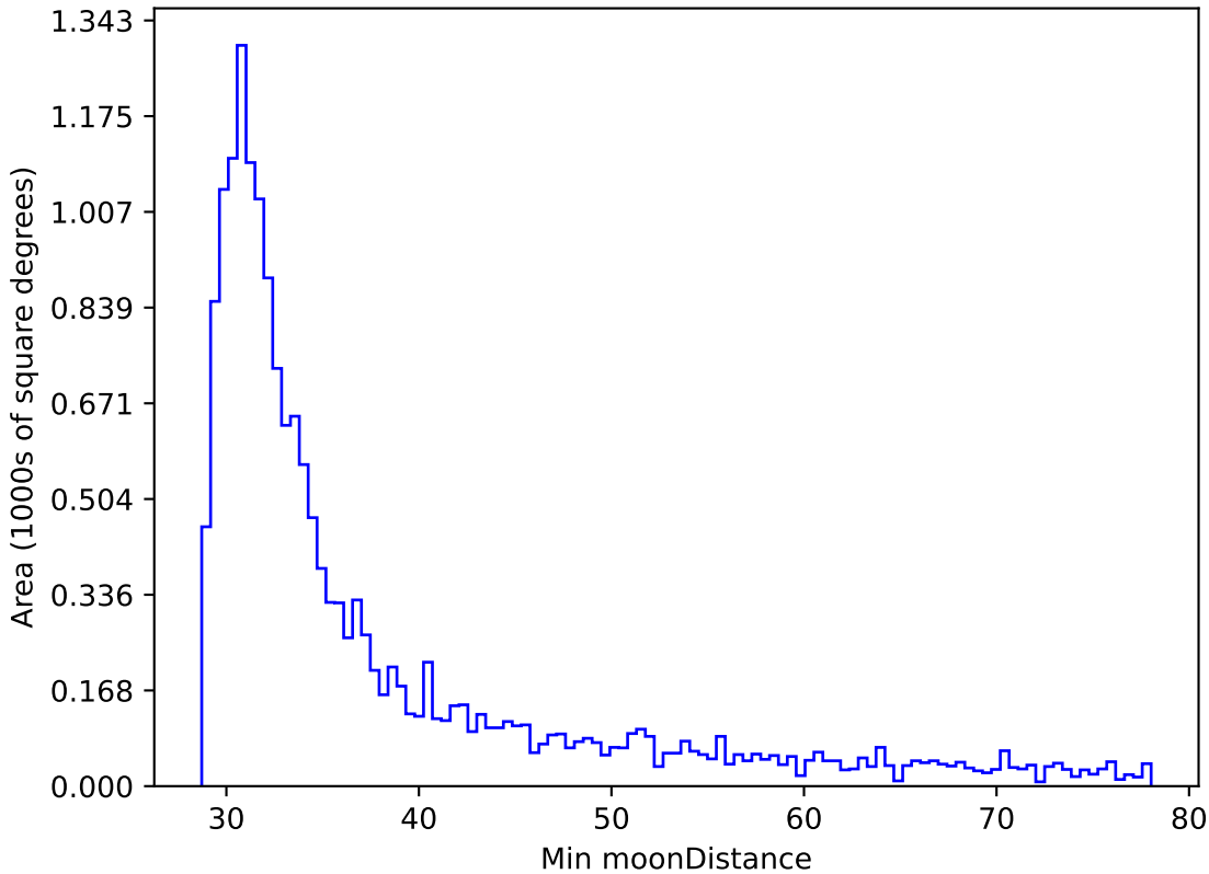
ddf_loaded_fl8_v3.4_10yrs WFD r band: Min moonDistance
