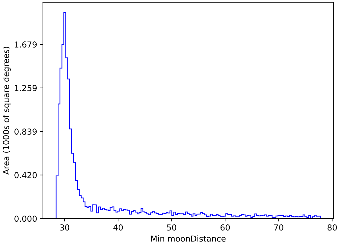
ddf_loaded_fl8_v3.4_10yrs WFD i band: Min moonDistance
