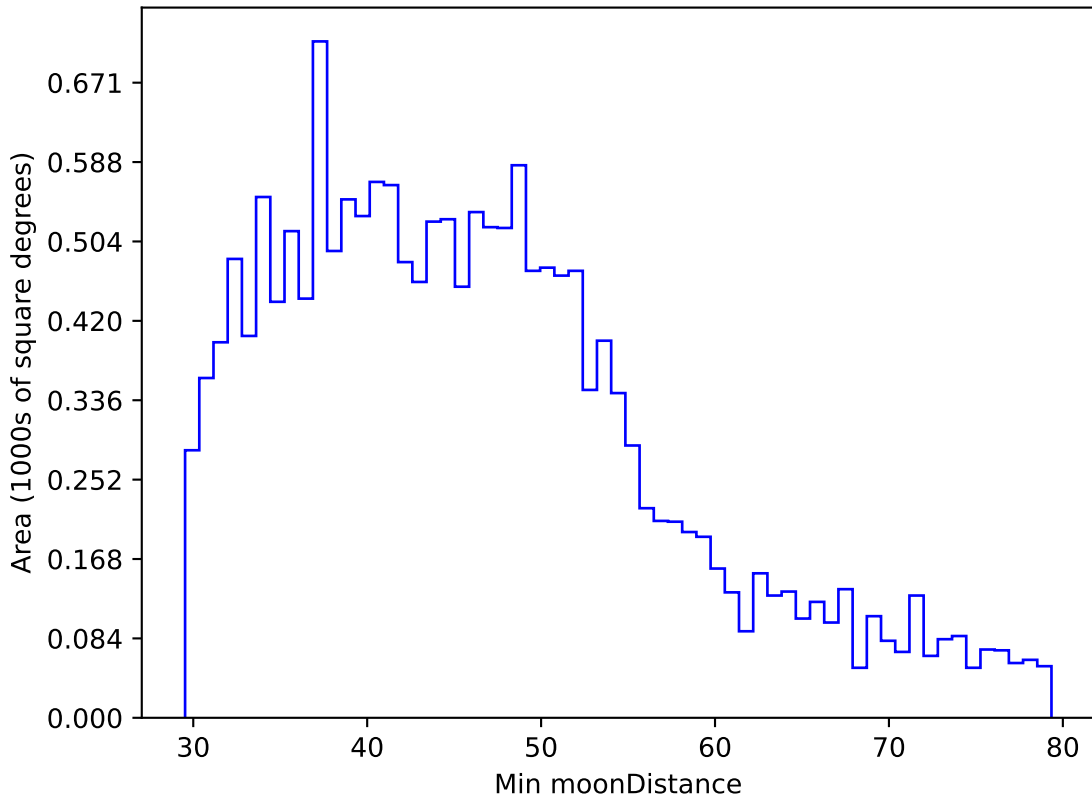
ddf_loaded_fl8_v3.4_10yrs WFD g band: Min moonDistance
