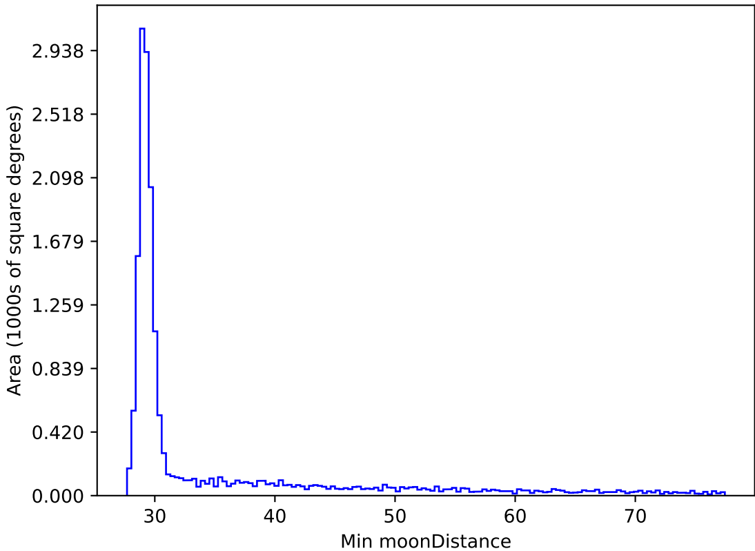
ddf_loaded_fl8_v3.4_10yrs WFD all bands: Min moonDistance
