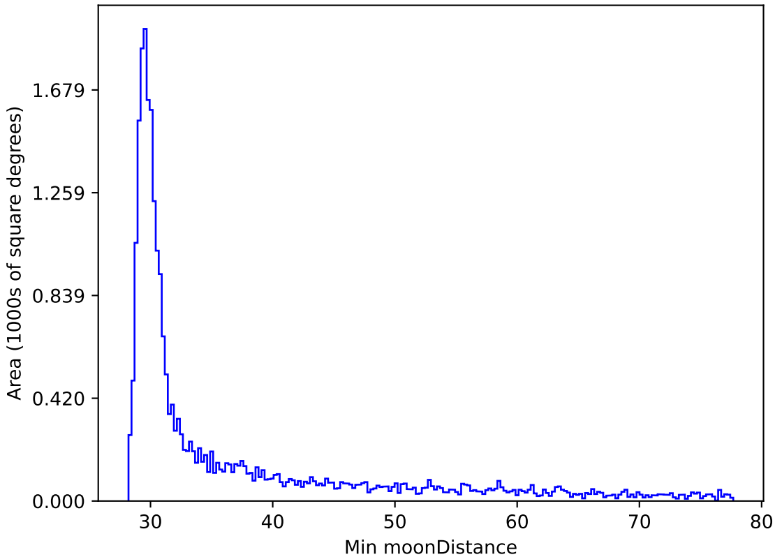
ddf_loaded_fl8_v3.4_10yrs All sky z band: Min moonDistance
