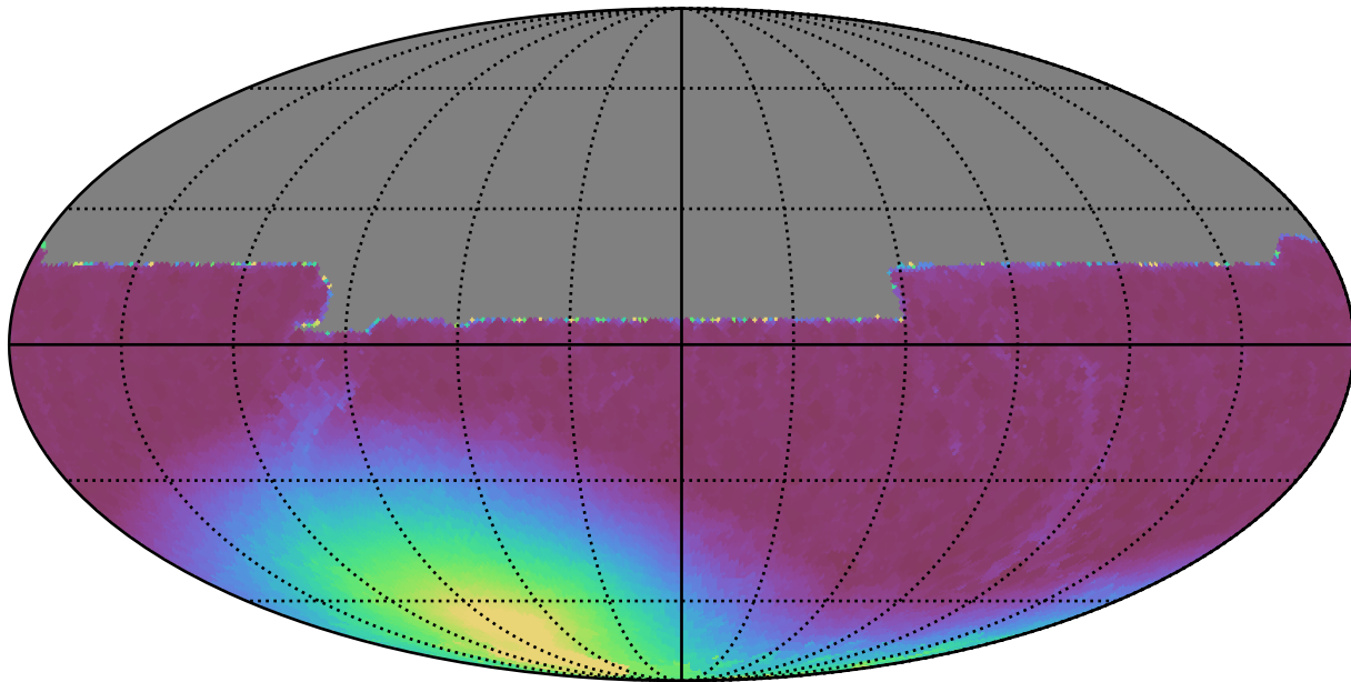
ddf_loaded_fl8_v3.4_10yrs All sky y band: Min moonDistance
