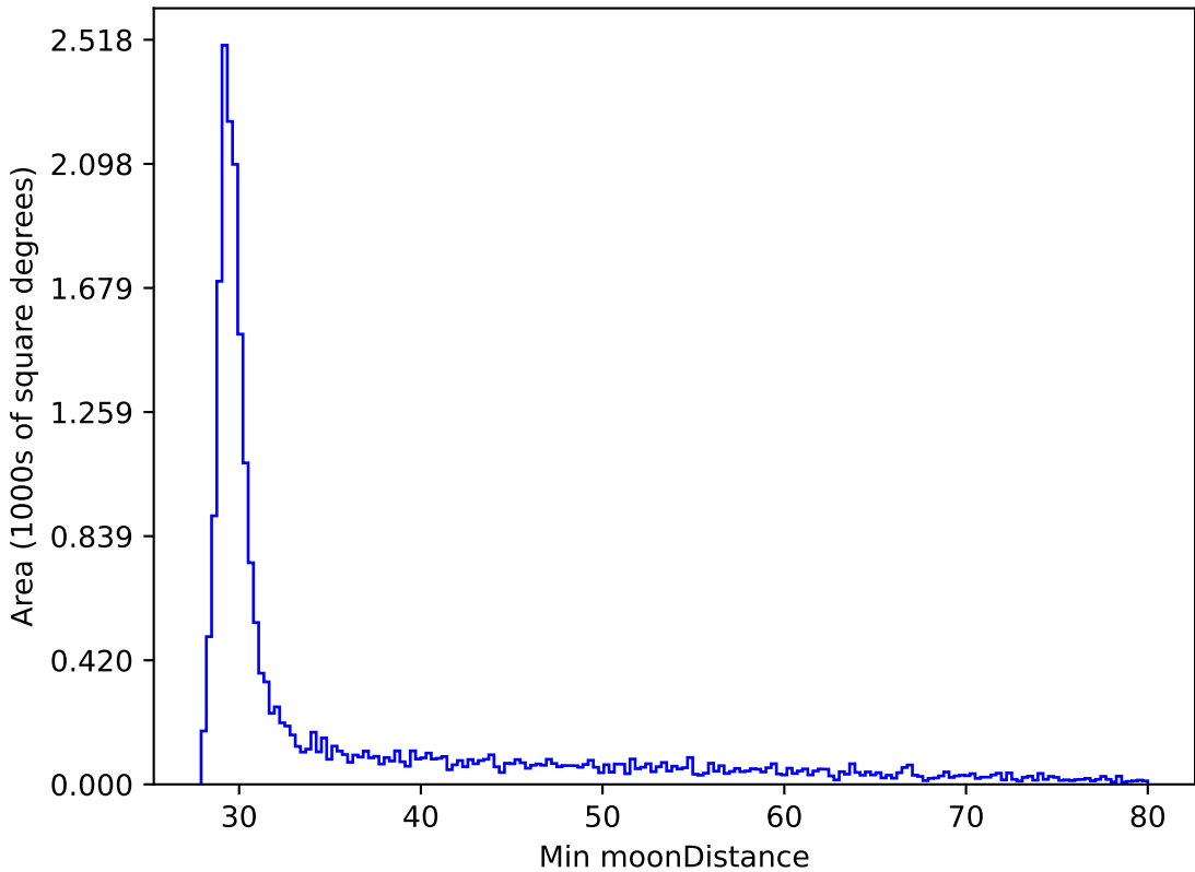
ddf_loaded_fl8_v3.4_10yrs All sky y band: Min moonDistance
