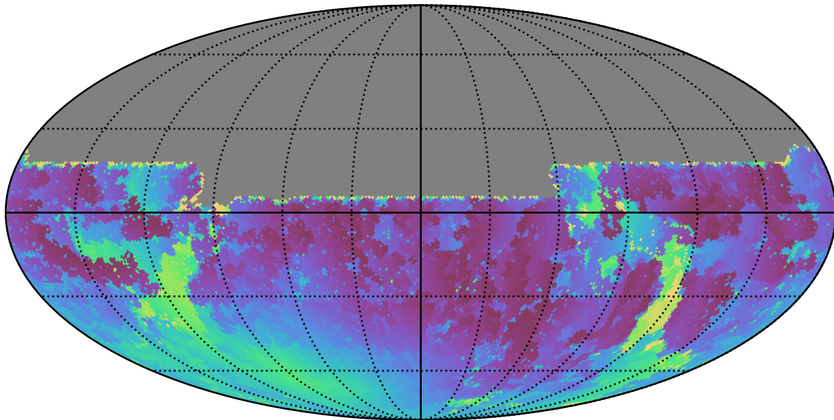
ddf_loaded_fl8_v3.4_10yrs All sky u band: Min moonDistance
