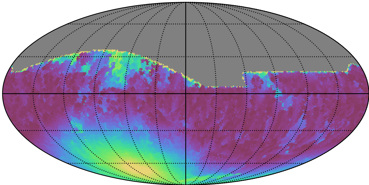
ddf_loaded_fl8_v3.4_10yrs All sky r band: Min moonDistance
