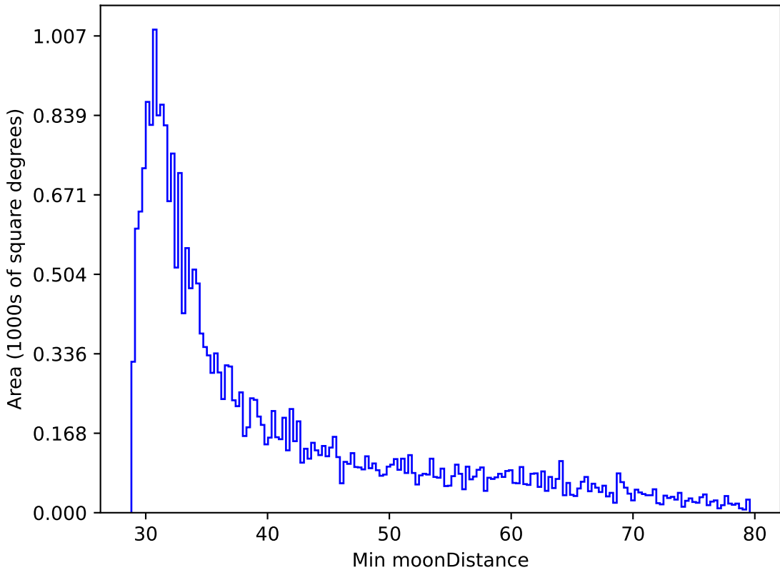
ddf_loaded_fl8_v3.4_10yrs All sky r band: Min moonDistance
