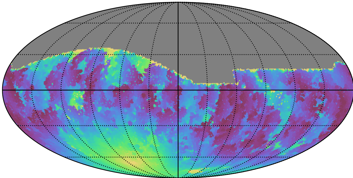
ddf_loaded_fl8_v3.4_10yrs All sky g band: Min moonDistance
