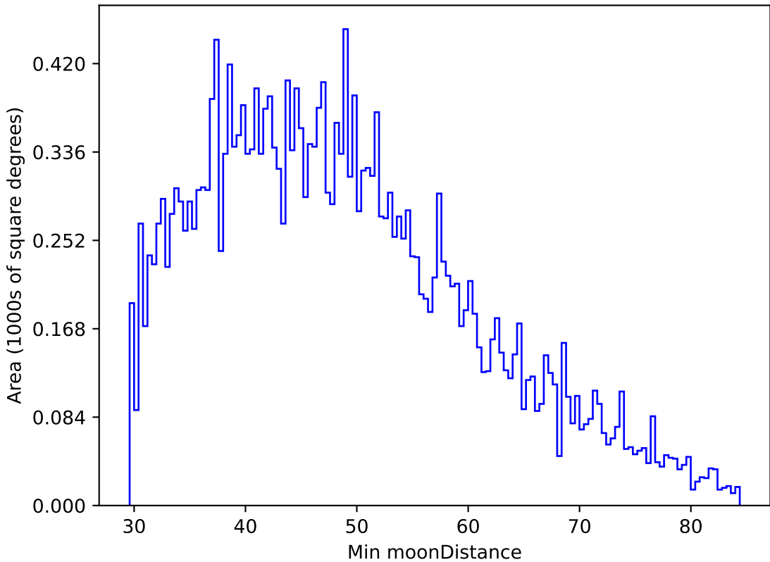
ddf_loaded_fl8_v3.4_10yrs All sky g band: Min moonDistance
