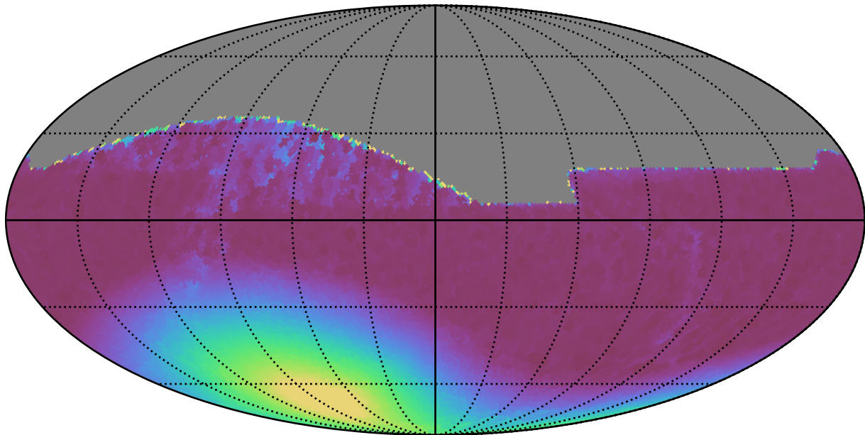
ddf_loaded_fl8_v3.4_10yrs All sky all bands: Min moonDistance
