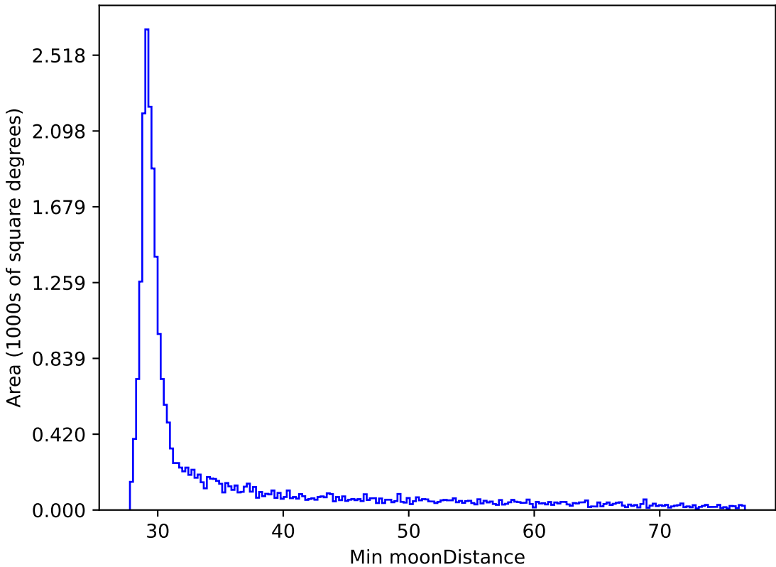
ddf_loaded_fl8_v3.4_10yrs All sky all bands: Min moonDistance
