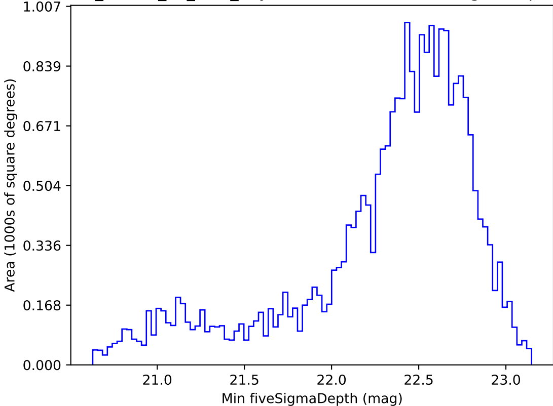
ddf_loaded_fl8_v3.4_10yrs Yr 1 z band: Min fiveSigmaDepth
