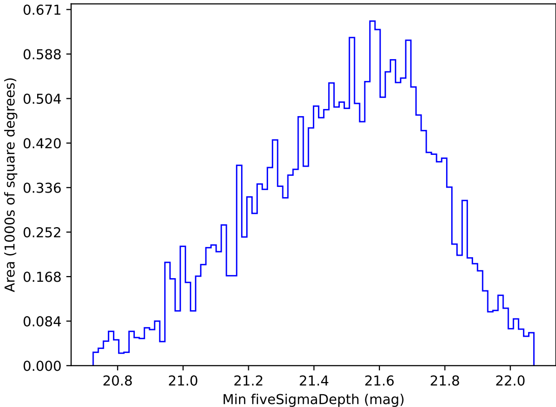
ddf_loaded_fl8_v3.4_10yrs Yr 1 y band: Min fiveSigmaDepth
