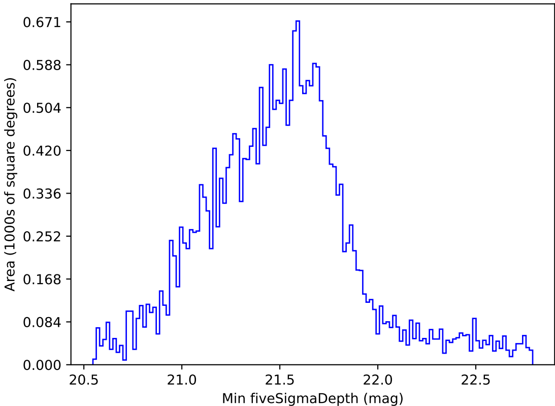
ddf_loaded_fl8_v3.4_10yrs Yr 1 all bands: Min fiveSigmaDepth
