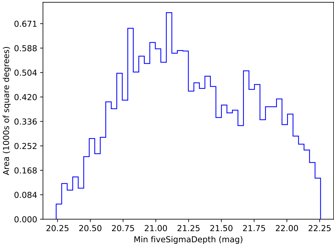
ddf_loaded_fl8_v3.4_10yrs WFD z band: Min fiveSigmaDepth
