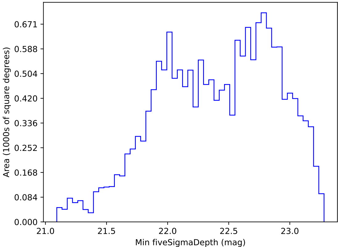
ddf_loaded_fl8_v3.4_10yrs WFD r band: Min fiveSigmaDepth
