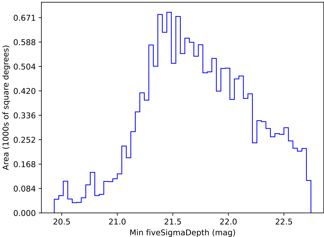
ddf_loaded_fl8_v3.4_10yrs WFD i band: Min fiveSigmaDepth
