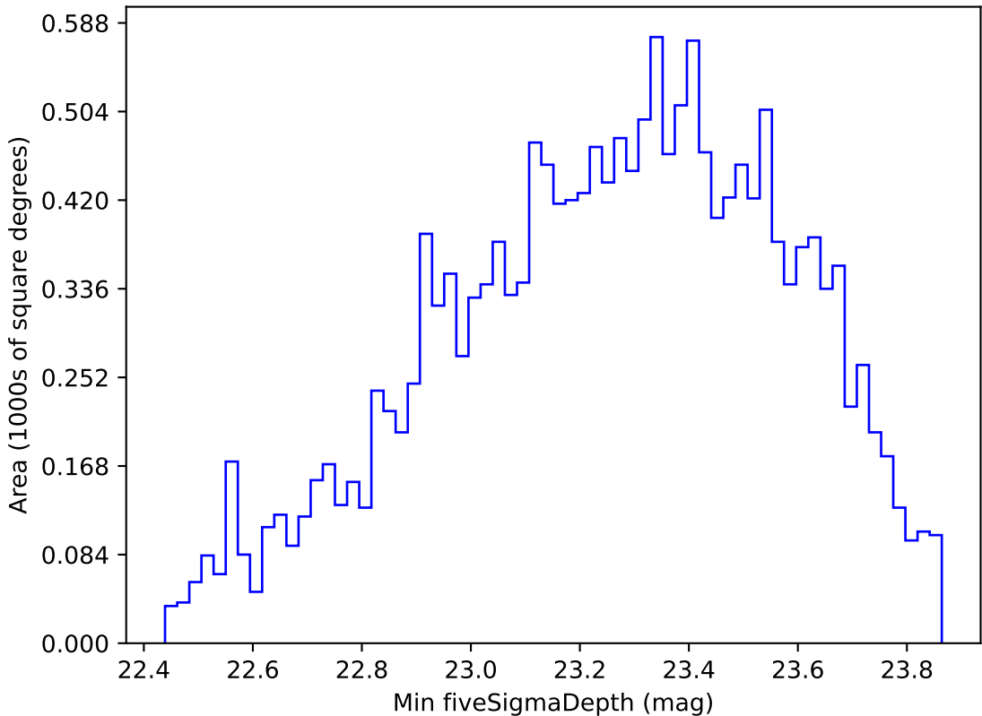
ddf_loaded_fl8_v3.4_10yrs WFD g band: Min fiveSigmaDepth
