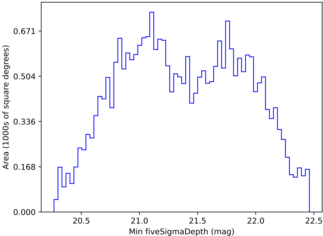
ddf_loaded_fl8_v3.4_10yrs All sky z band: Min fiveSigmaDepth
