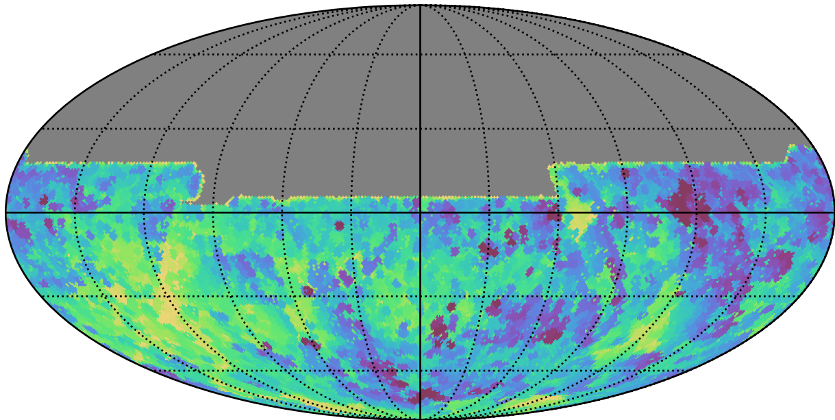
ddf_loaded_fl8_v3.4_10yrs All sky y band: Min fiveSigmaDepth
