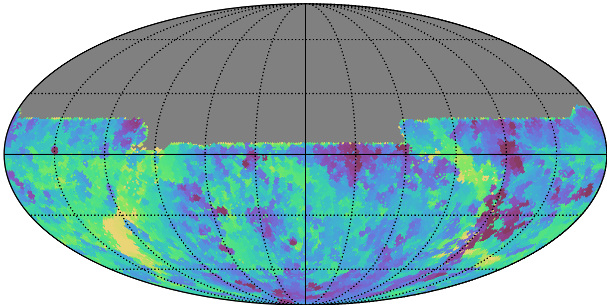
ddf_loaded_fl8_v3.4_10yrs All sky u band: Min fiveSigmaDepth
