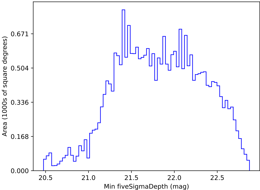
ddf_loaded_fl8_v3.4_10yrs All sky i band: Min fiveSigmaDepth
