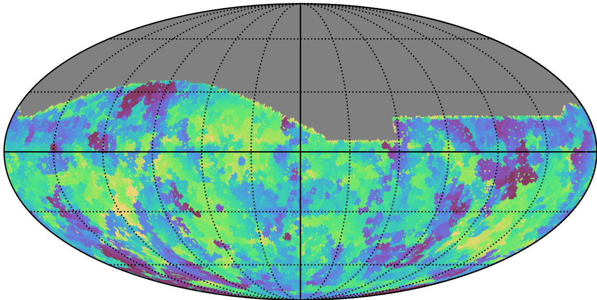
ddf_loaded_fl8_v3.4_10yrs All sky g band: Min fiveSigmaDepth
