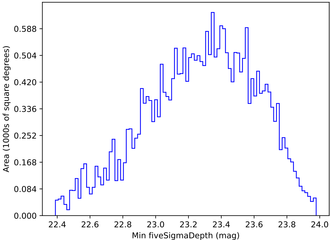
ddf_loaded_fl8_v3.4_10yrs All sky g band: Min fiveSigmaDepth
