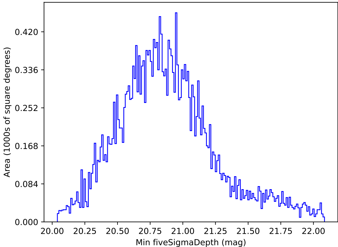
ddf_loaded_fl8_v3.4_10yrs All sky all bands: Min fiveSigmaDepth
