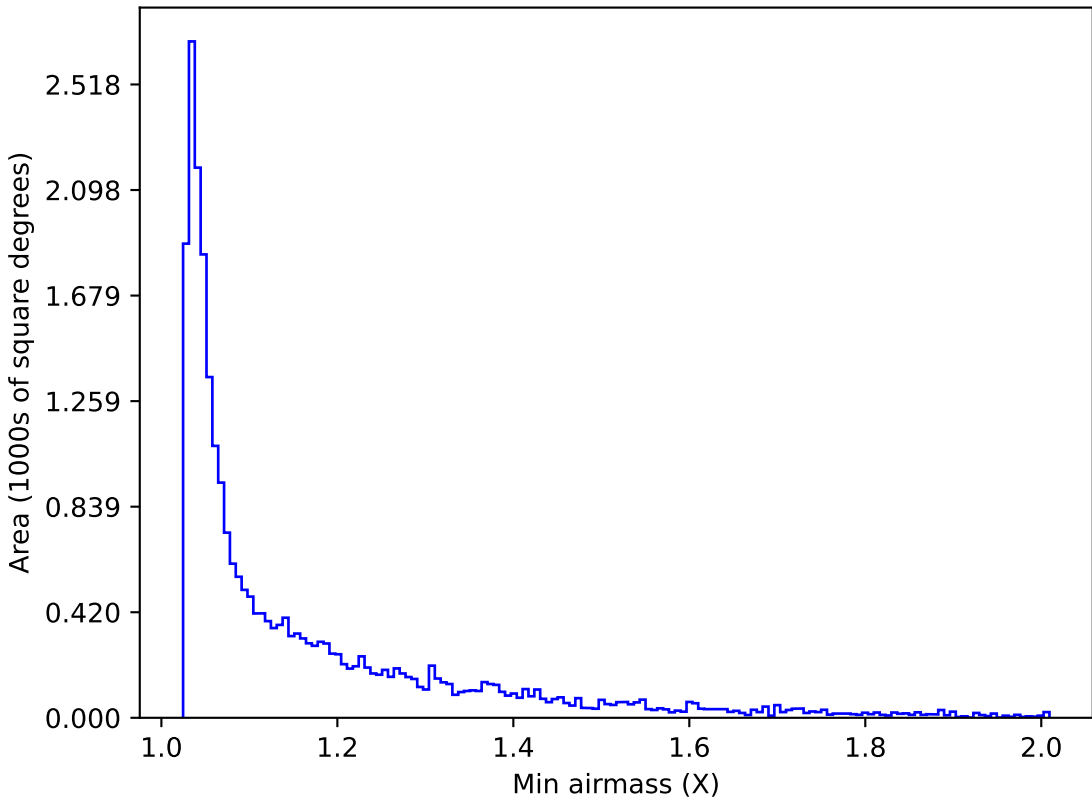
ddf_loaded_fl8_v3.4_10yrs Yr 1 z band: Min airmass
