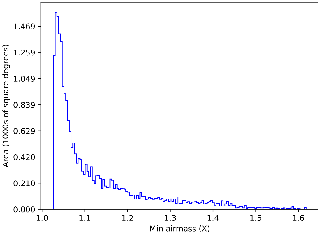
ddf_loaded_fl8_v3.4_10yrs Yr 1 y band: Min airmass
