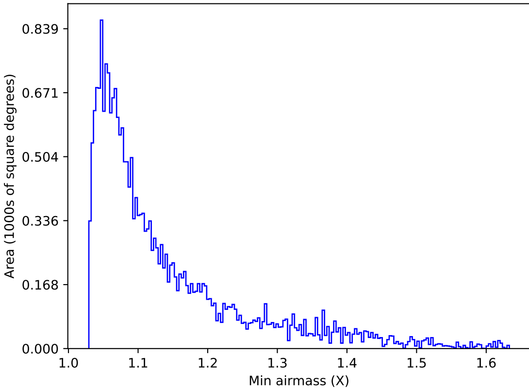
ddf_loaded_fl8_v3.4_10yrs Yr 1 u band: Min airmass
