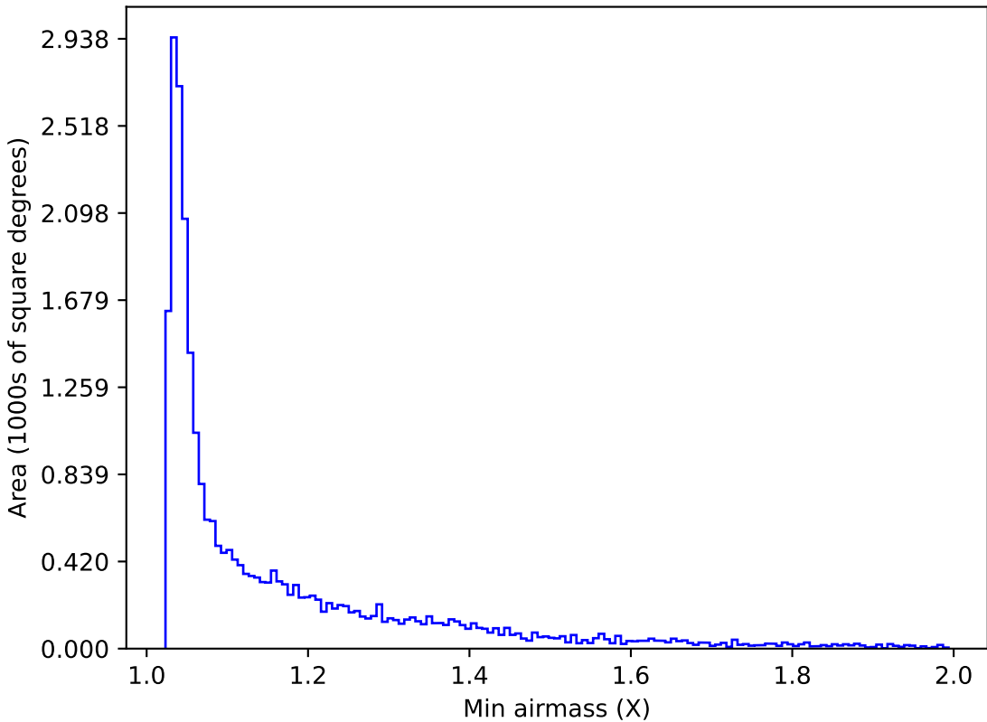
ddf_loaded_fl8_v3.4_10yrs Yr 1 r band: Min airmass
