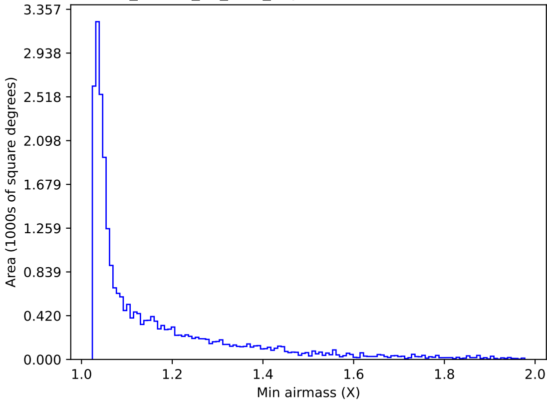
ddf_loaded_fl8_v3.4_10yrs Yr 1 i band: Min airmass
