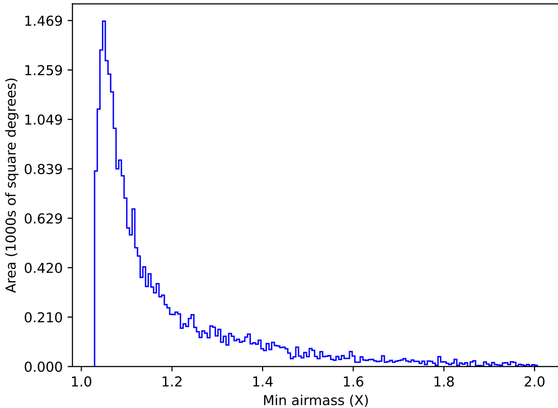
ddf_loaded_fl8_v3.4_10yrs Yr 1 g band: Min airmass
