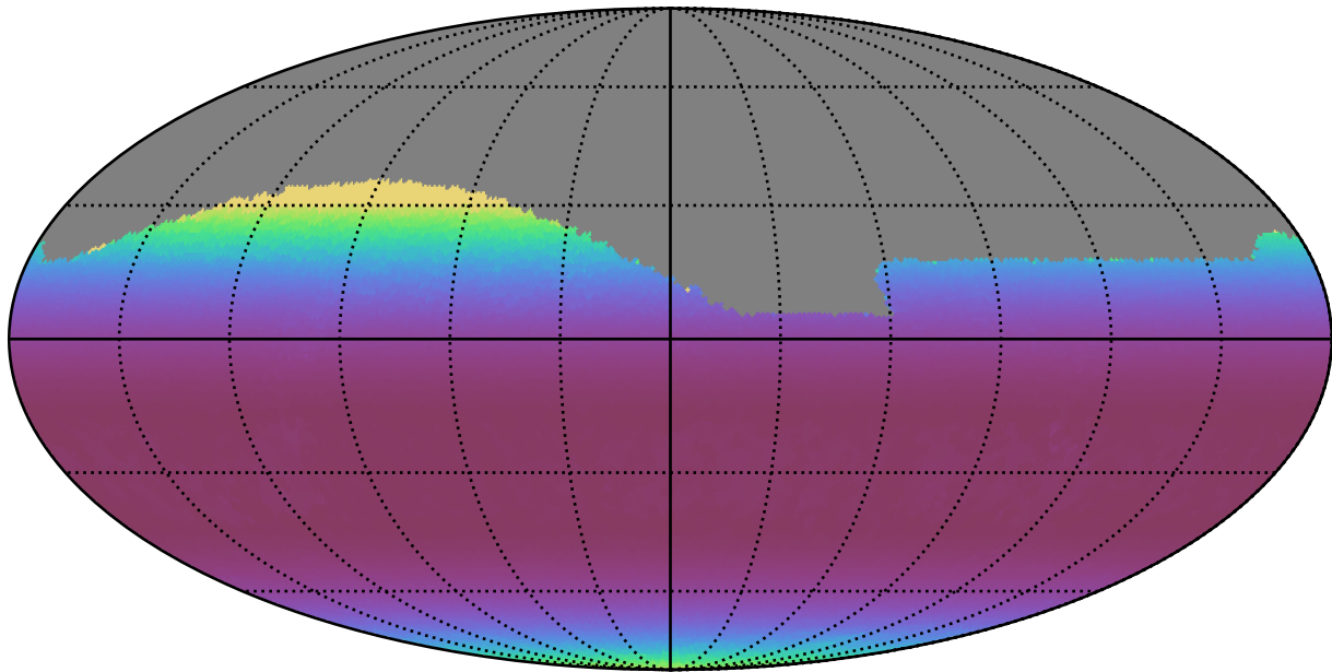
ddf_loaded_fl8_v3.4_10yrs Yr 1 all bands: Min airmass
