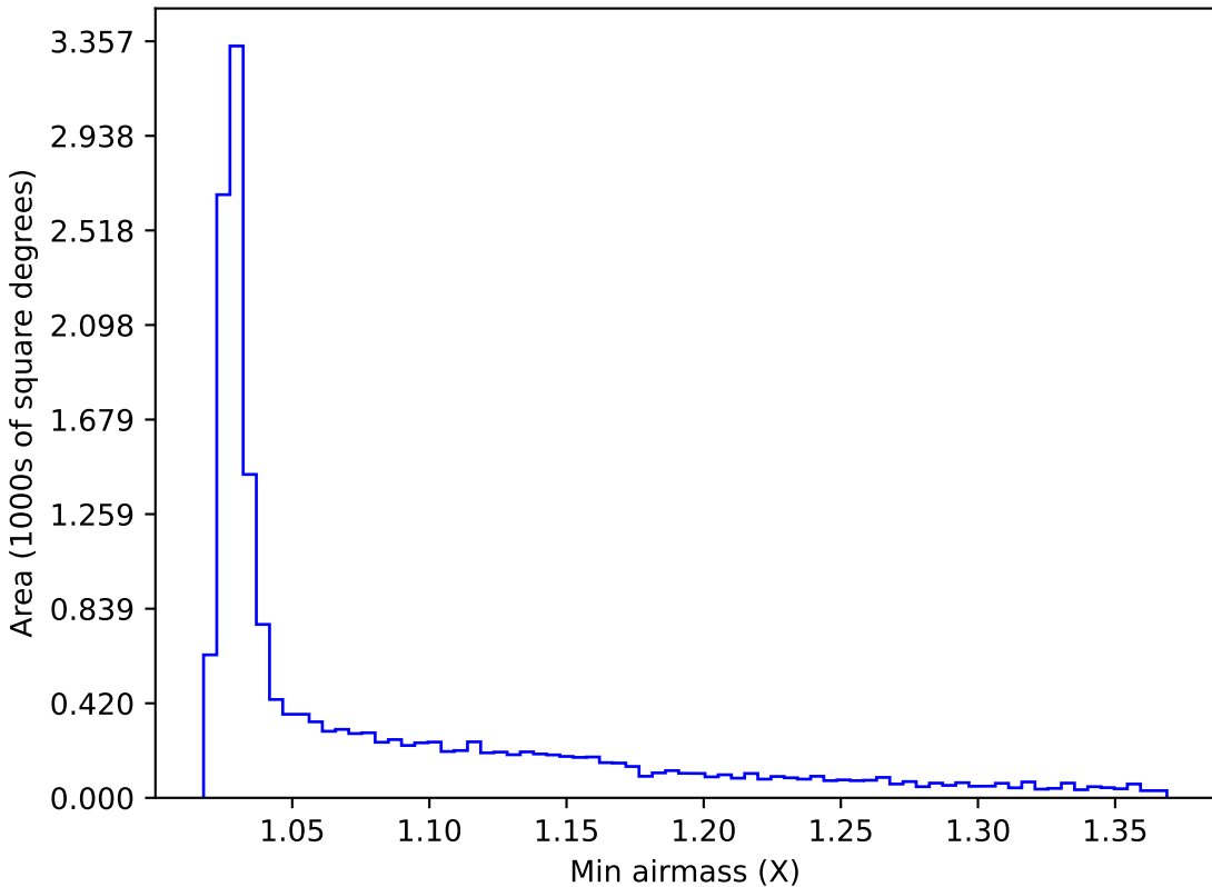
ddf_loaded_fl8_v3.4_10yrs WFD z band: Min airmass
