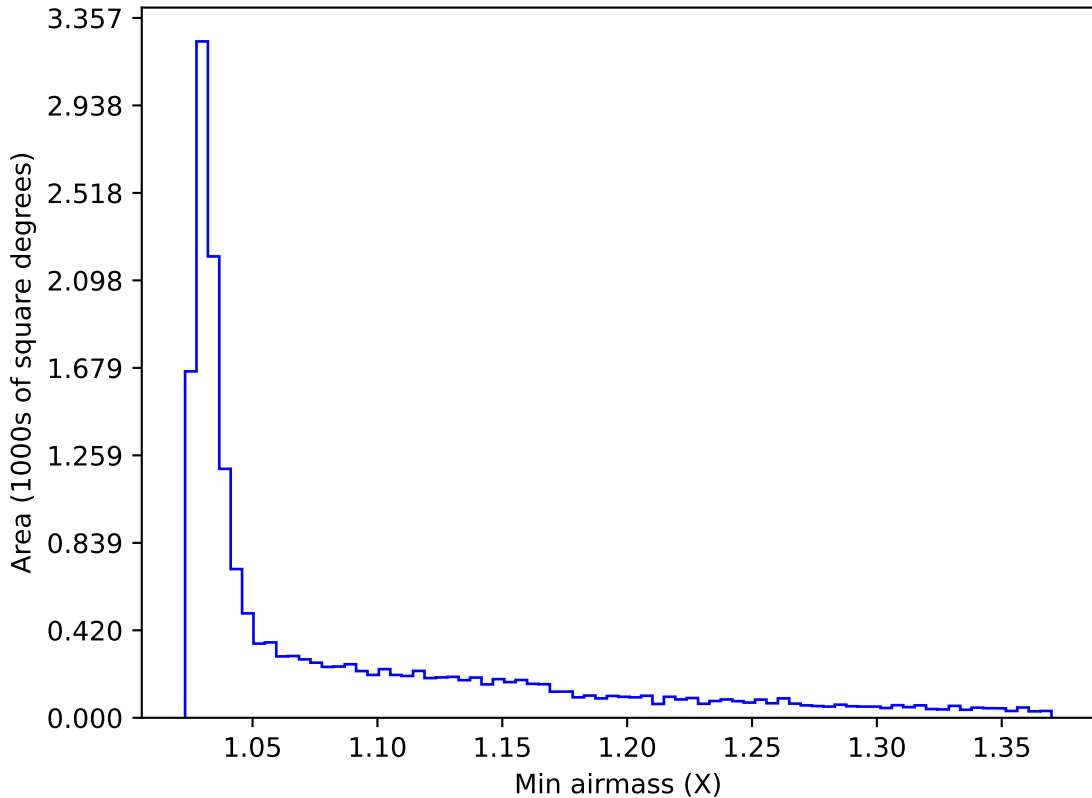
ddf_loaded_fl8_v3.4_10yrs WFD y band: Min airmass
