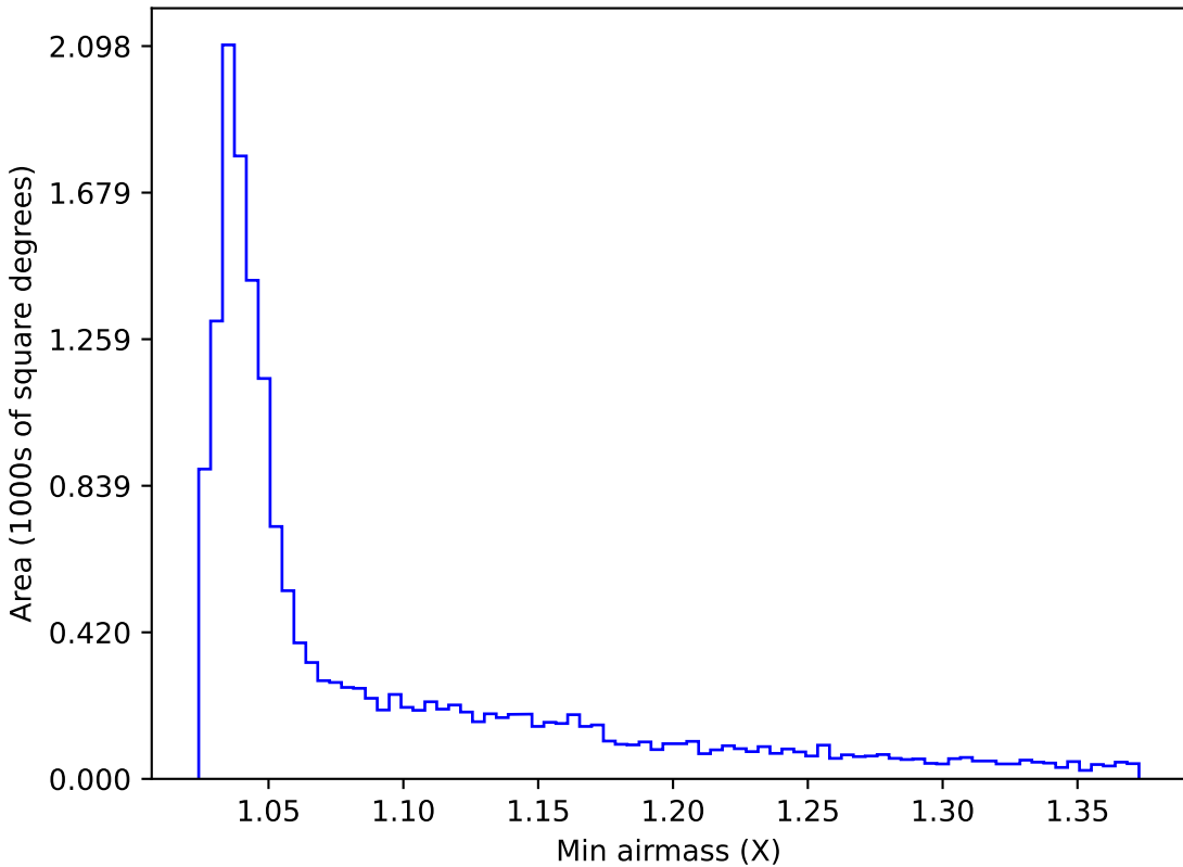
ddf_loaded_fl8_v3.4_10yrs WFD u band: Min airmass
