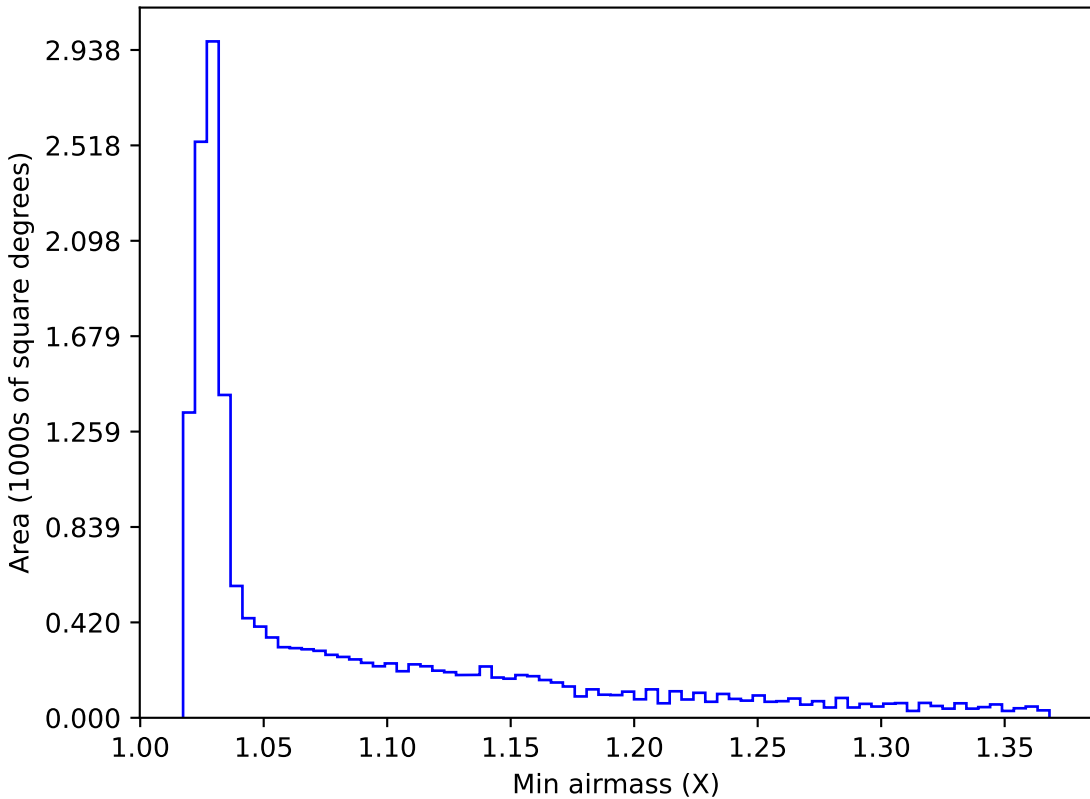
ddf_loaded_fl8_v3.4_10yrs WFD r band: Min airmass
