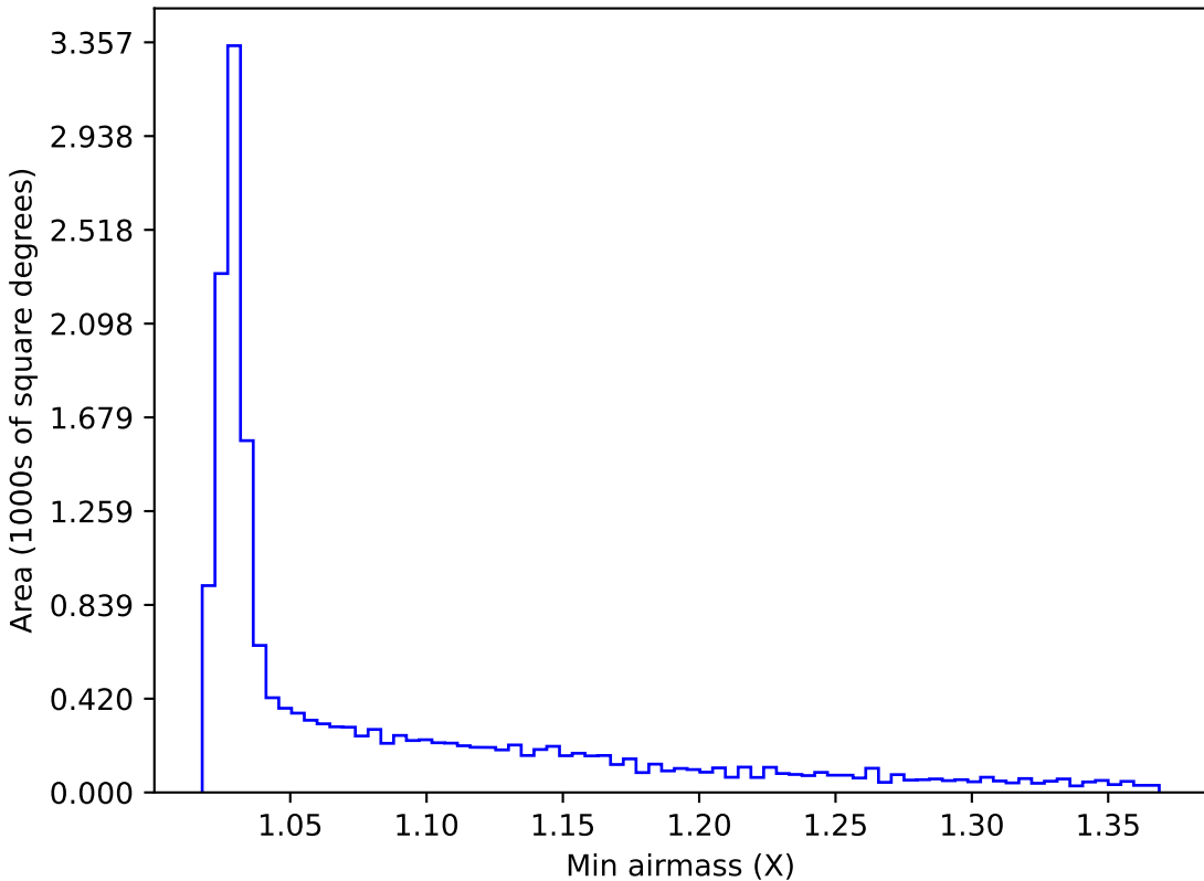
ddf_loaded_fl8_v3.4_10yrs WFD i band: Min airmass
