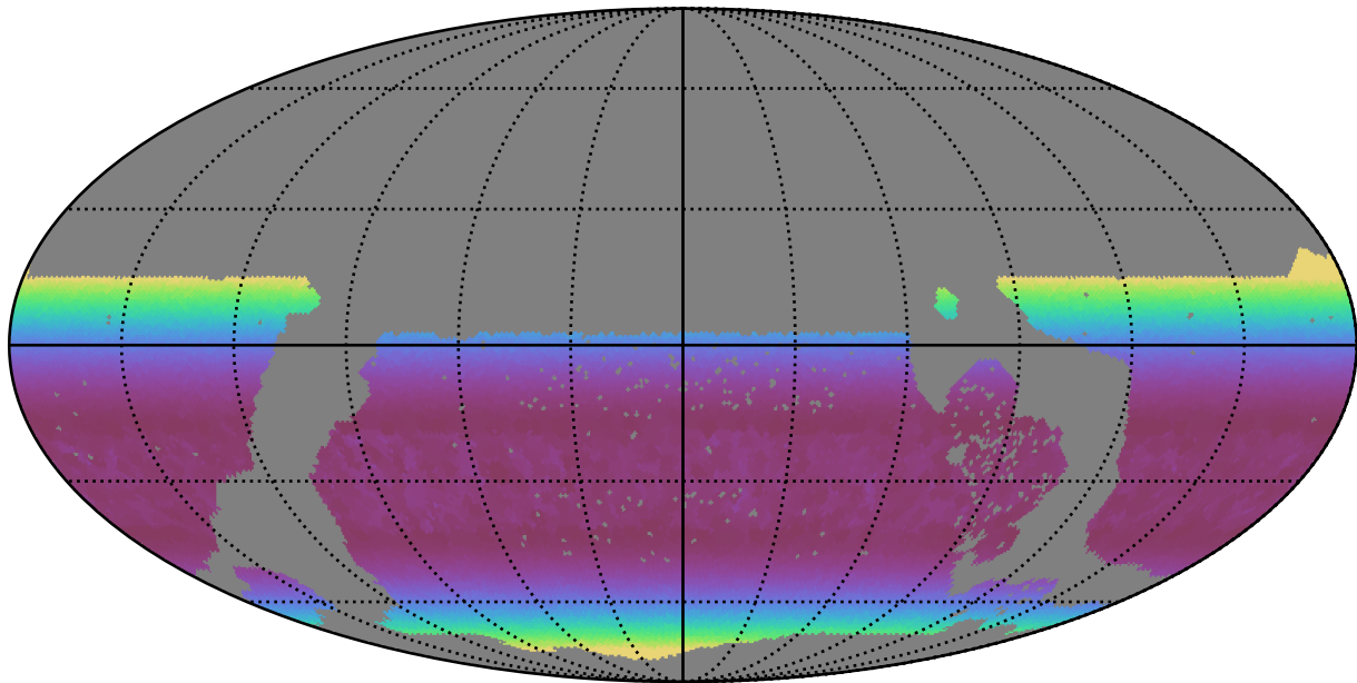
ddf_loaded_fl8_v3.4_10yrs WFD g band: Min airmass
