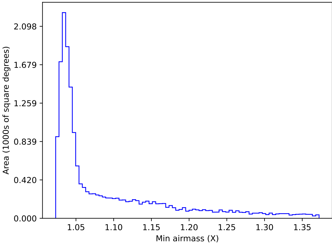
ddf_loaded_fl8_v3.4_10yrs WFD g band: Min airmass
