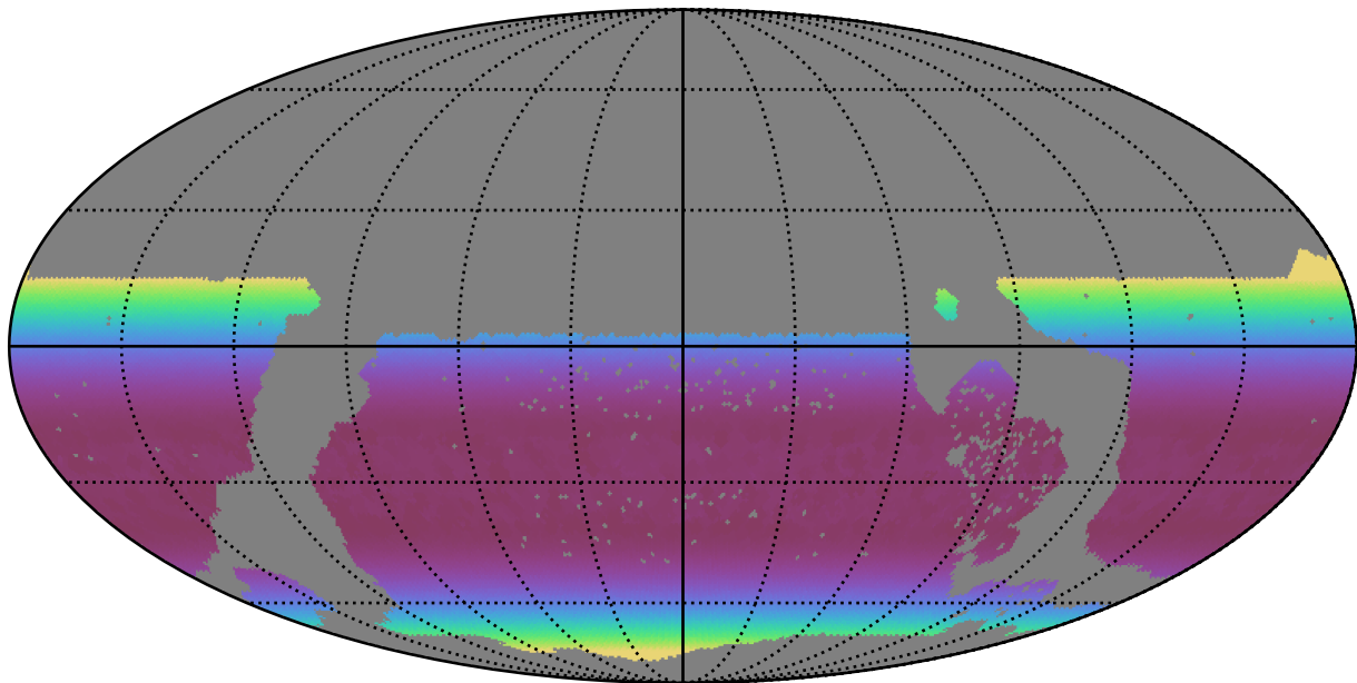
ddf_loaded_fl8_v3.4_10yrs WFD all bands: Min airmass
