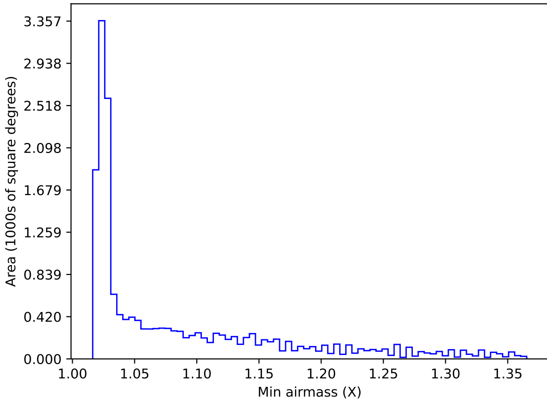
ddf_loaded_fl8_v3.4_10yrs WFD all bands: Min airmass
