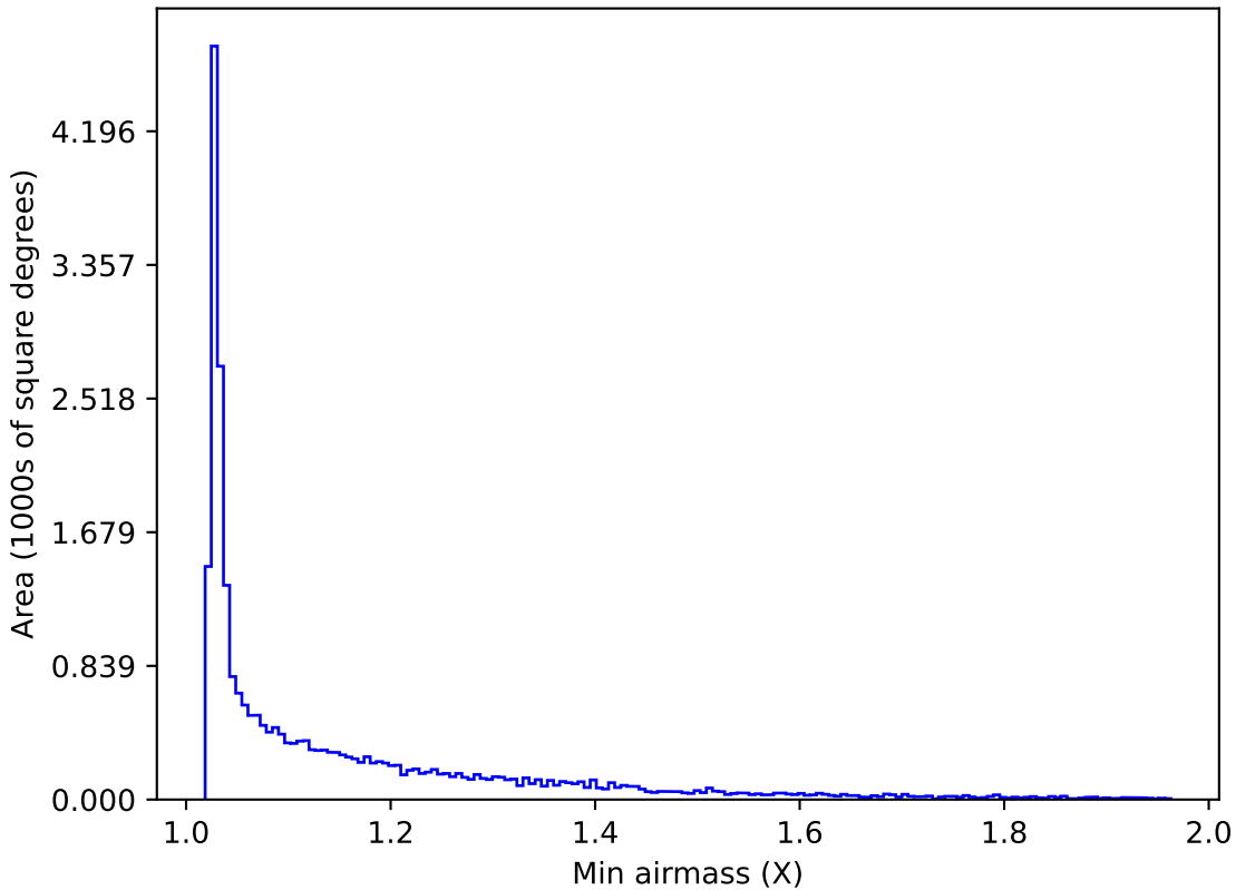
ddf_loaded_fl8_v3.4_10yrs All sky z band: Min airmass
