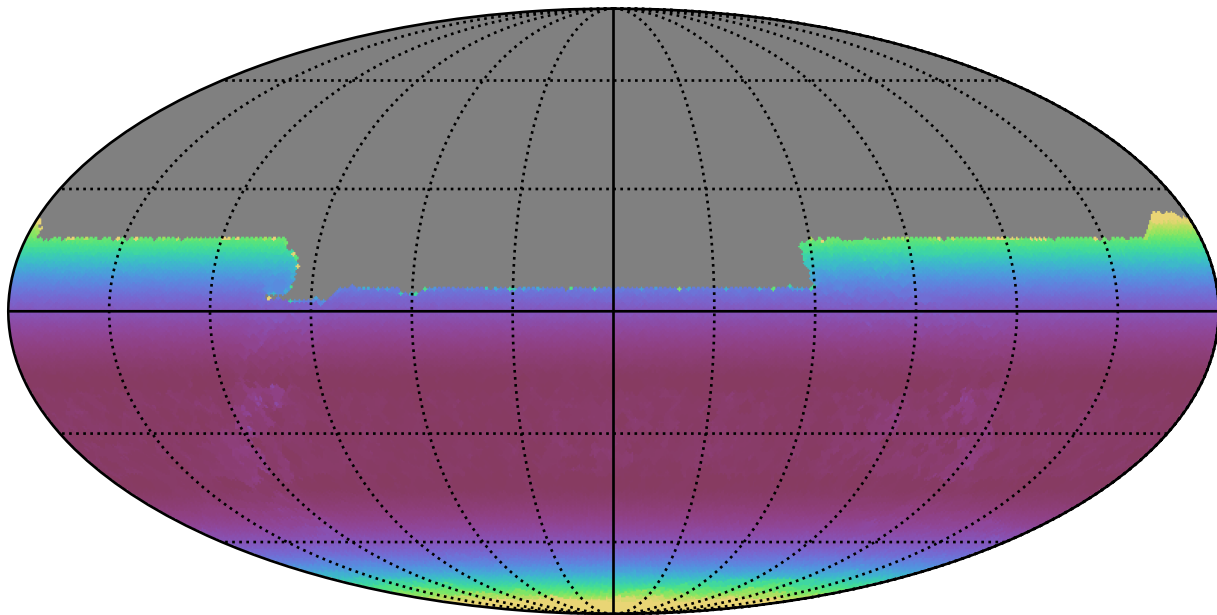
ddf_loaded_fl8_v3.4_10yrs All sky y band: Min airmass
