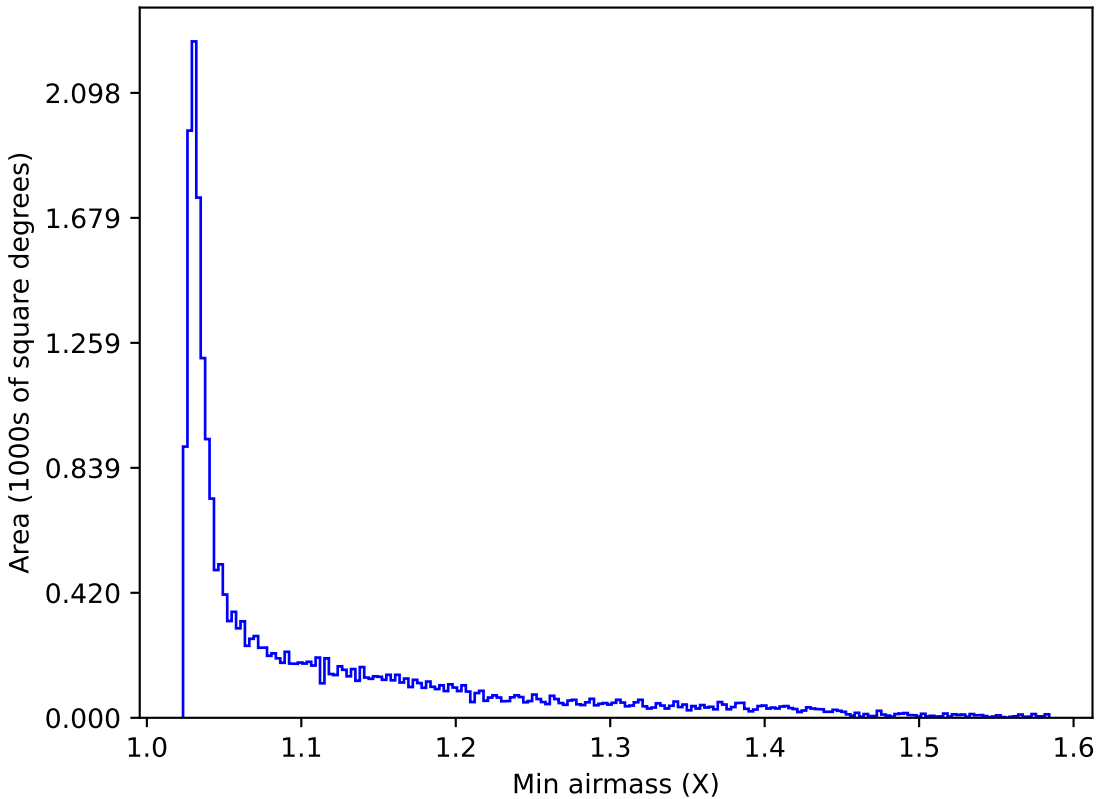
ddf_loaded_fl8_v3.4_10yrs All sky y band: Min airmass
