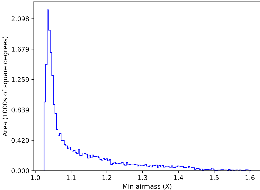
ddf_loaded_fl8_v3.4_10yrs All sky u band: Min airmass
