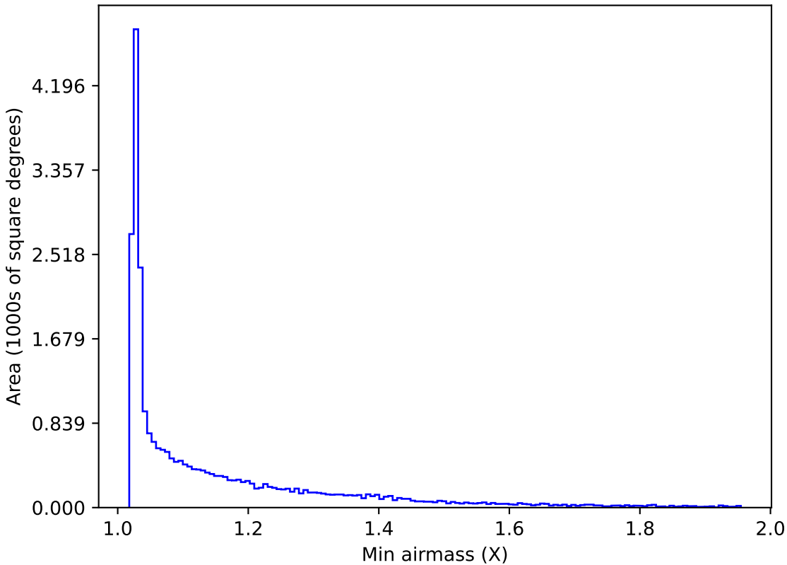
ddf_loaded_fl8_v3.4_10yrs All sky r band: Min airmass
